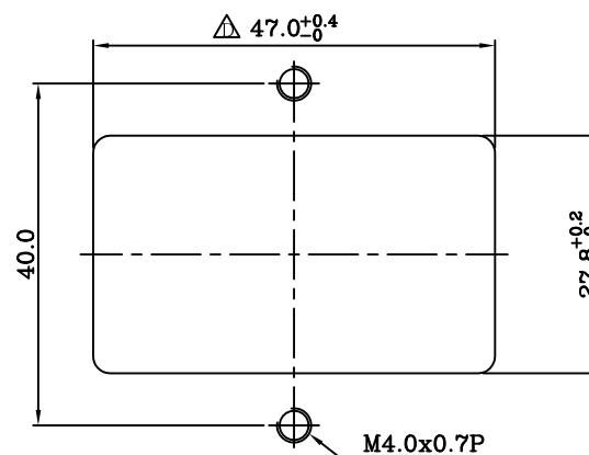
PANEL CUT-OUT
