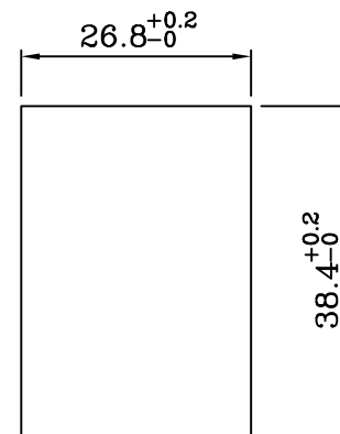
PANEL CUT-OUT
