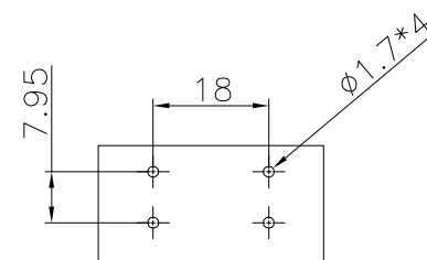
PCB LAYOYT(1:1)
