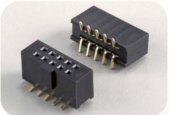
Female Header Dual Row SMT (with Bump)
