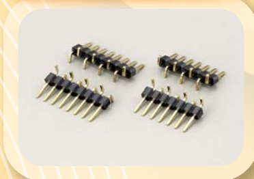
Pin Header Single Row SMT
