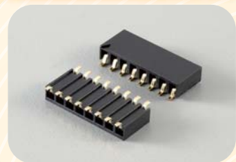
Female Header Single Row SMT Side Entry
