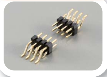
Pin Header Dual Row SMT Side Entry
