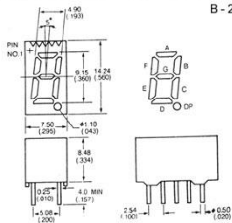
PIN CONNECTION
