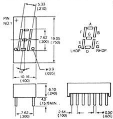
PIN CONNECTION
