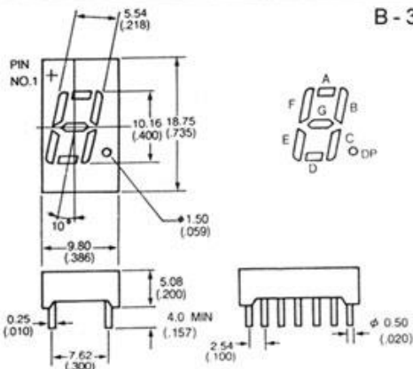
PIN CONNECTION
