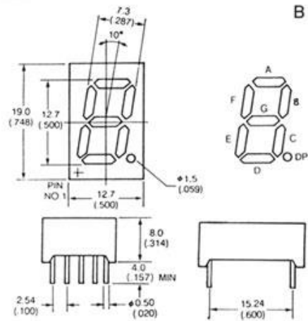
PIN CONNECTION
