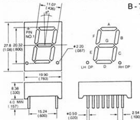
PIN CONNECTION
