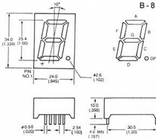
PIN CONNECTION
