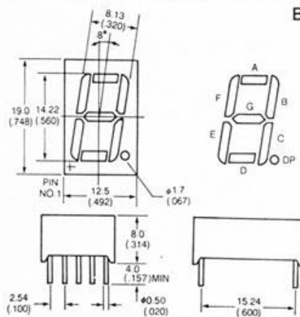
PIN CONNECTION
