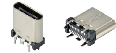
317D(F7) USB Type C Receptacle Vertical Height:10.5mm Positions:24
