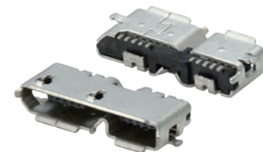
317D(D2) micro USB 3.0 B SMT Positions:10
