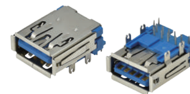
377A(F1) USB 3.1 A Receptacle (Power delivery available) Positions:10
