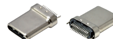
317C(F2) USB Type C Plug Extrusion Dual SMT Positions:24
